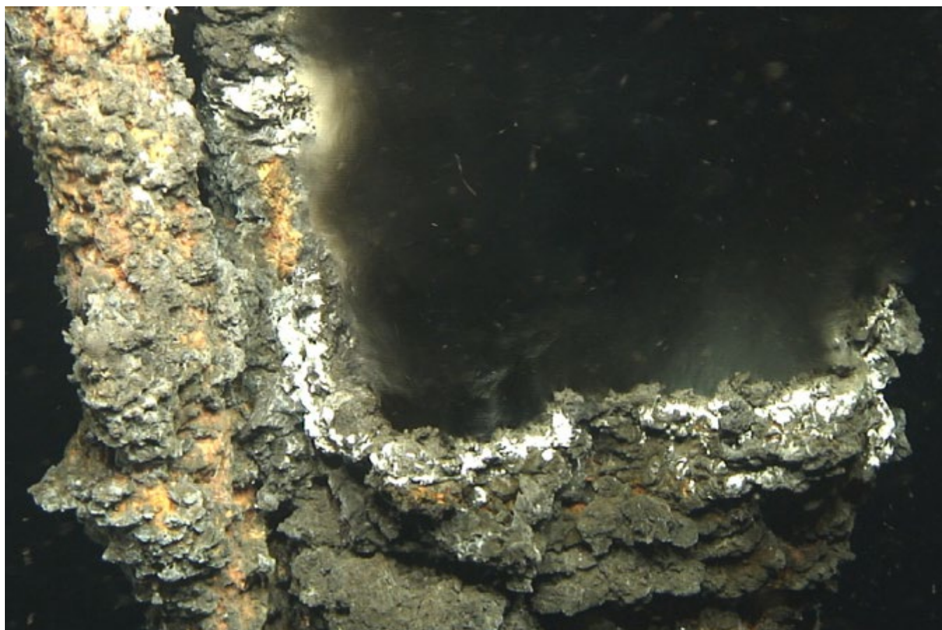
Black, metal-rich water at 300°C flows from a so-called «chimney» on the seabed, 300 km west of Bear Island. Deposits of copper, zinc and gold with a value of NOK 1 - 5 billion have been proved along the Mid-Oceanic Ridge in the middle of the Atlantic. Photo: Centre of Excellence in Geobiology
